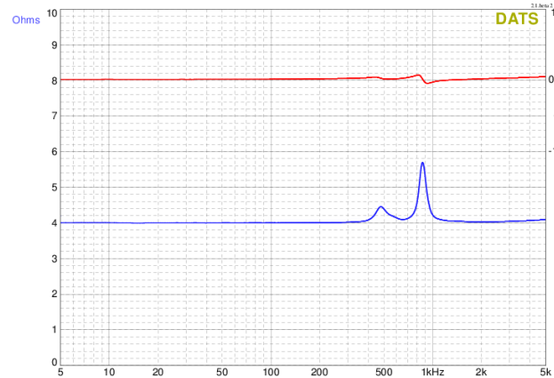
Measurement taken with transducer uncoupled facing upward.
