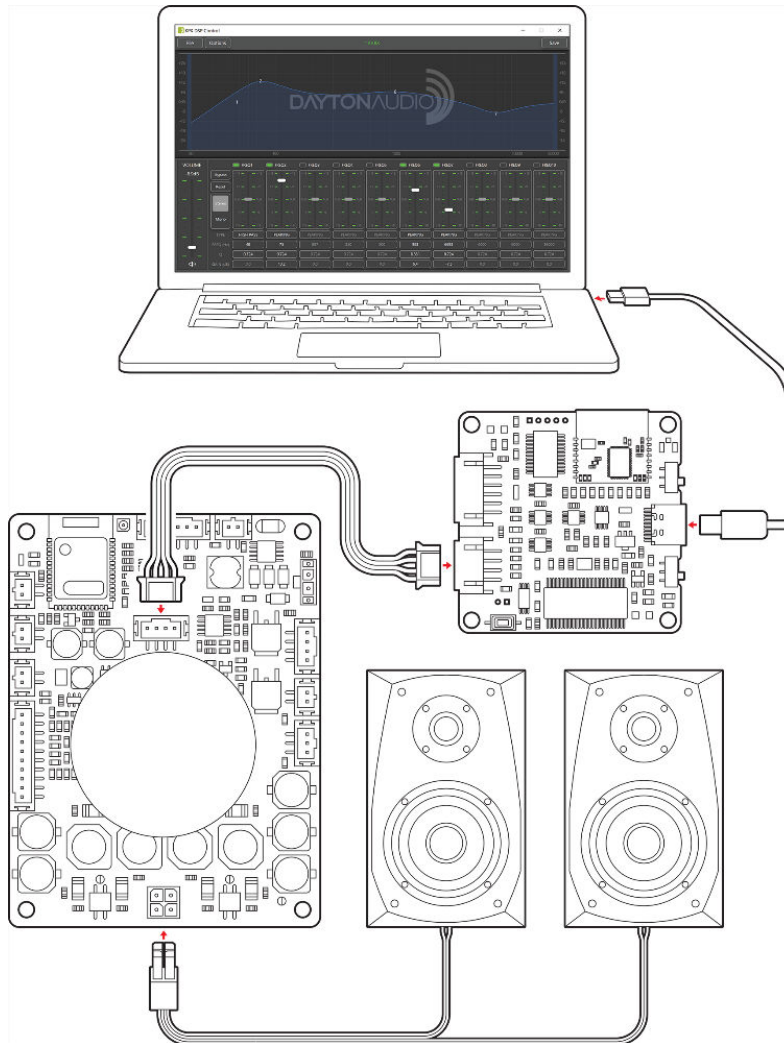
Pictured is a KAB-250v4 amplifier connected to the KPX programmer, which is connected to a Windows laptop running the KABX software.
