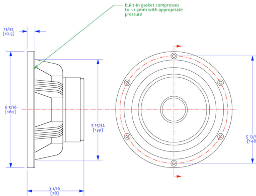
Alpair 10.2 no bezel cover driver dimensions drawn by did | 24 June 2011
