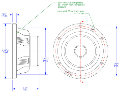
Alpair 10.2 with bezel cover driver dimensions drawn by did | 24 June 2011
