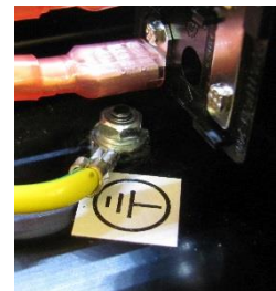
Earth connection
