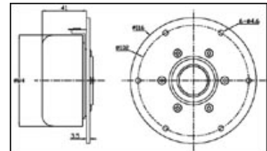
Mechanical Drawing (Magnify)
