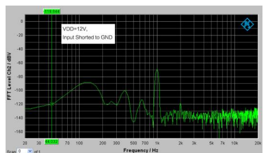
Noise Floor
