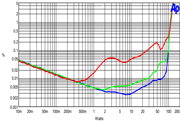
THD+N vs. Po at 100Hz, 1kHz and 6.67kHz 8) (8Ω), 230Vac/50Hz
