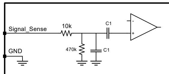
Figure 12: Signal_Sense input
