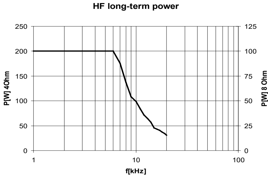
Figure 5: HF long-term output power
