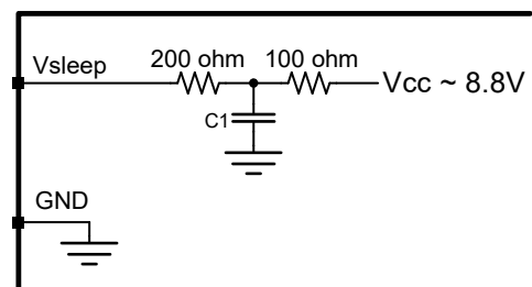
Figure 13: Vsleep output
