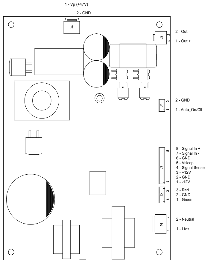
Figure 1: ICEpower200ASC connections
