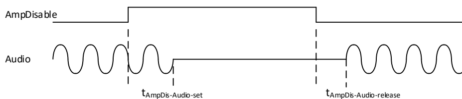
Figure 20: Standby and AmpDisable timing
